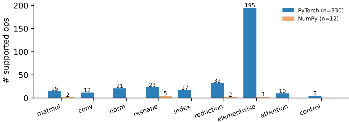
TensorGuard operator coverage by family
