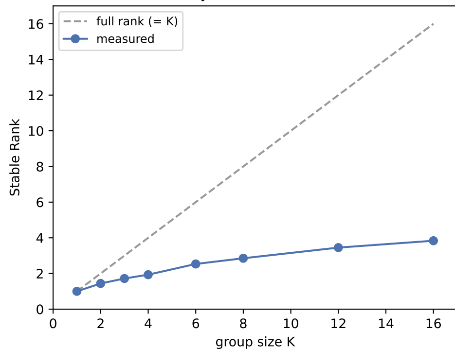
Analytic block-SVD-OMP
