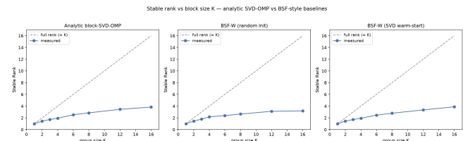
Figure 2: Stable rank vs. block size K on activations. All three methods (analytic SVD-OMP blocks, cold-init BSF-W, SVD-warm-started BSF-W) plateau below the dashed full-rank = K line. Analytic SVD-OMP blocks track BSF-W-warm exactly.
