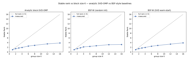
Figure 2: Stable rank vs. block size K on activations. All three methods (analytic SVD-OMP blocks, cold-init BSF-W, SVD-warm-started BSF-W) plateau below the dashed full-rank= K line. Analytic SVD-OMP blocks track BSF-W-warm exactly.
