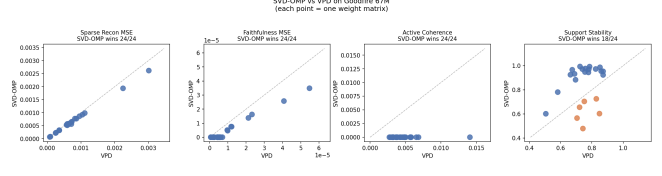
Figure 1: SVD-OMP vs. VPD on the 24 target modules. Each point is one weight matrix; below the y = x line means SVD-OMP wins. SVD-OMP wins every per-metric comparison 24 / 24 on sparse reconstruction, faithfulness, and coherence; and 18 / 24 on stability (all six losses are attention v_{proj} / o_{proj} ; see Sec. 4.1).
