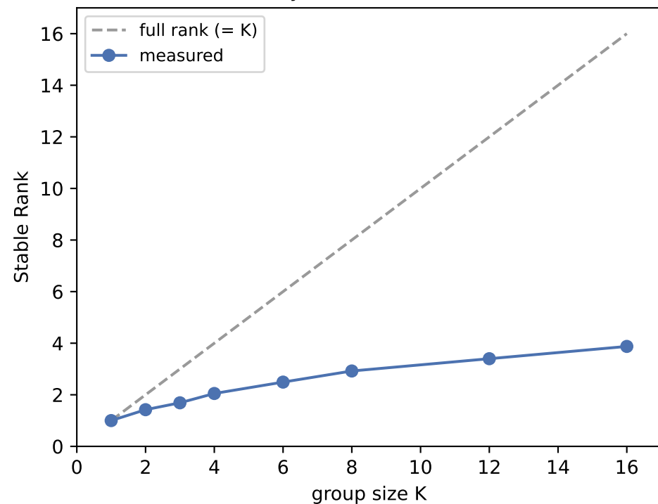
Analytic block-SVD-OMP
