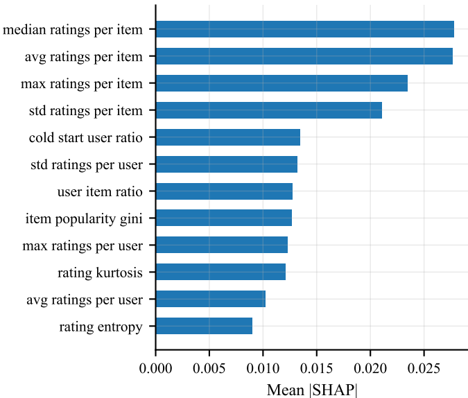
Feature importance
