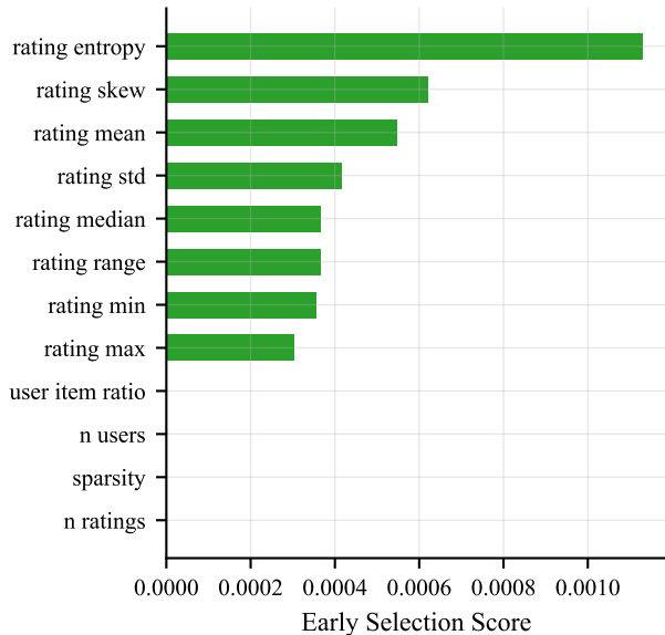
ESS ranking
