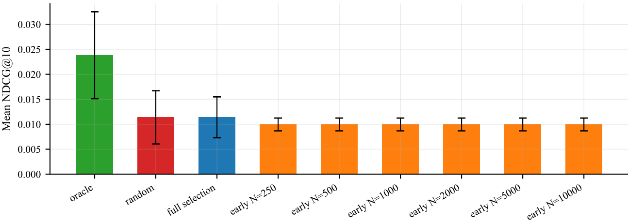
End-to-end recommendation quality by selection strategy
