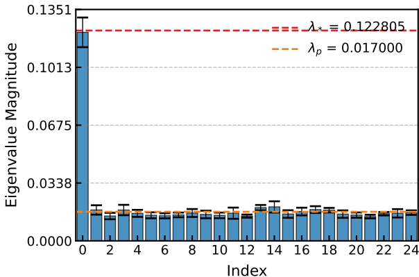
Eigenvalues of K_{\mu\nu} (N=250, P=30, D=25)
