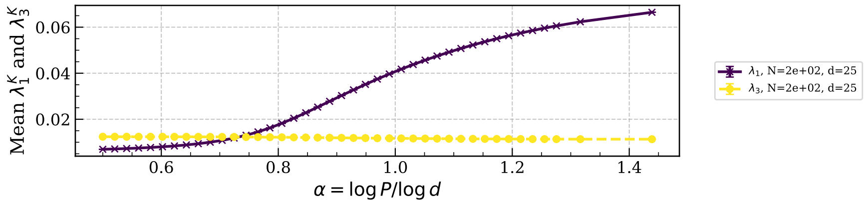
Mean \lambda_1^K and \lambda_3^K vs. \alpha
