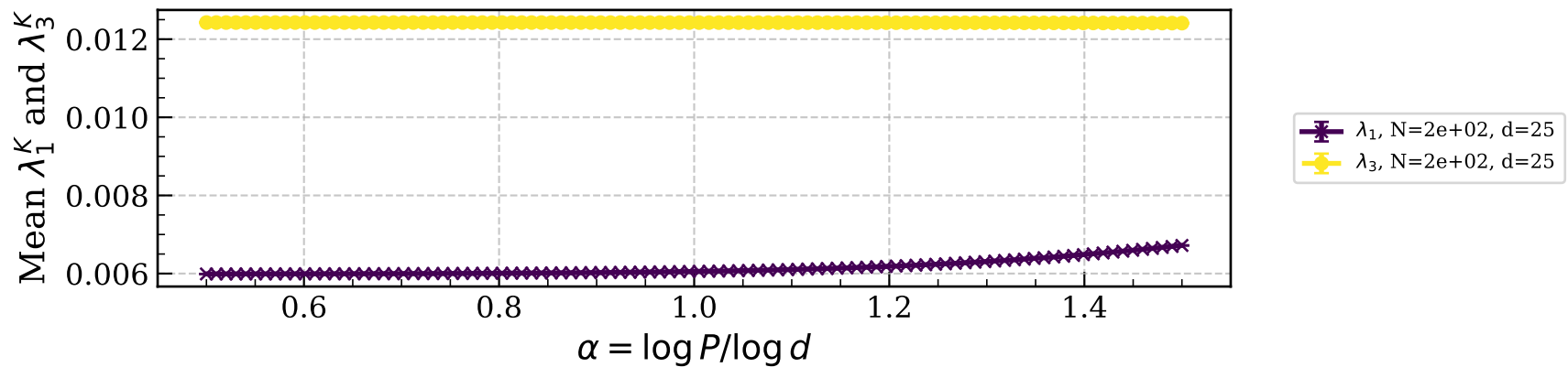
Mean \lambda_1^K and \lambda_3^K vs. \alpha
