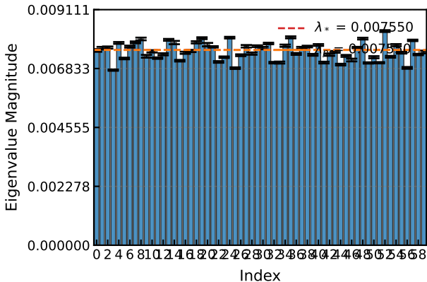
Eigenvalues of K_{\mu\nu} (N=600, P=80, D=60)
