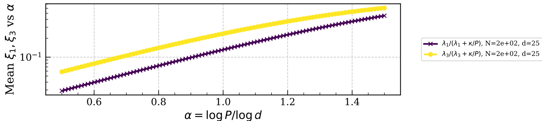
Mean \xi_1 and \xi_3 vs. \alpha
