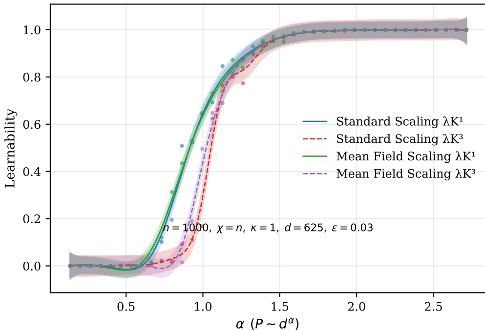
Learnability Scaling (Overlay)
