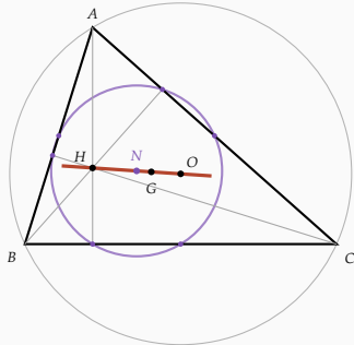
Euler line O, G, H with OG : GH = 1 : 2 ; nine-point circle (centre N = \text{midpoint of } OH , radius R/2 ) passes through the 3 feet of altitudes, 3 midpoints, and midpoints of AH, BH, CH .
