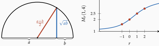
Left: \text{GM} \leq \text{AM} as altitude \leq radius. Right: M_r increases in r (HM, GM, AM, QM marked).
