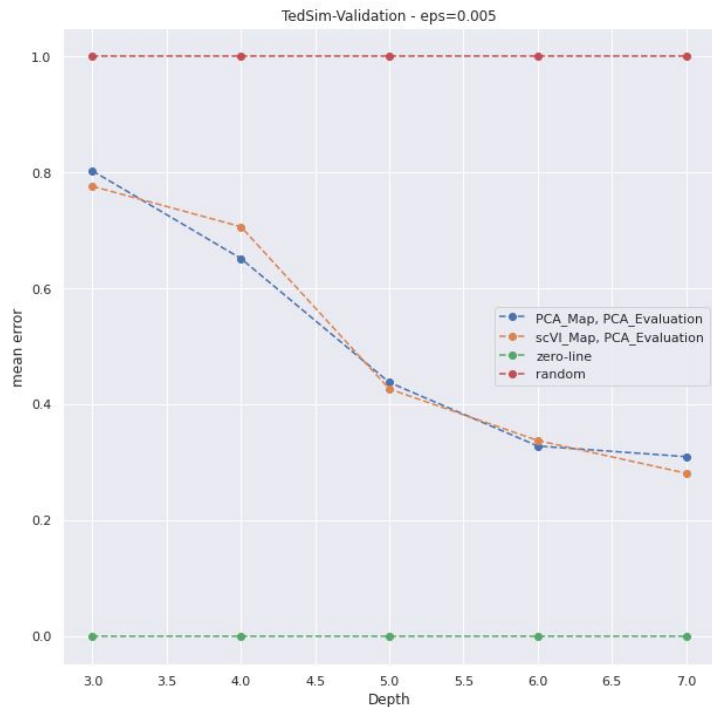
Evaluation in (30-dim.) PCA space ( i.e. mean error is calculated using PCA-cost matrix)
