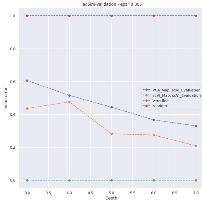
Evaluation in scVI latent space
