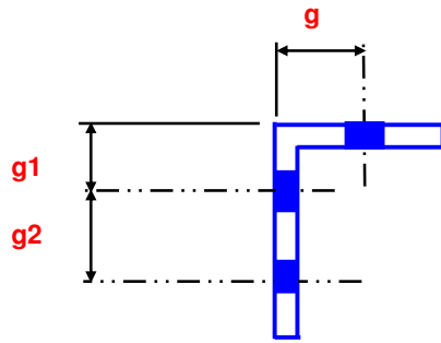
Usual Gages For Angles , Inches
