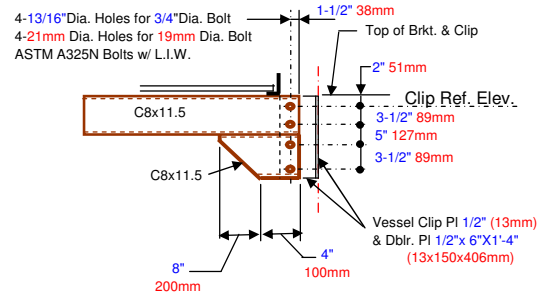
Typical Hot Vessel Bracket Detail
