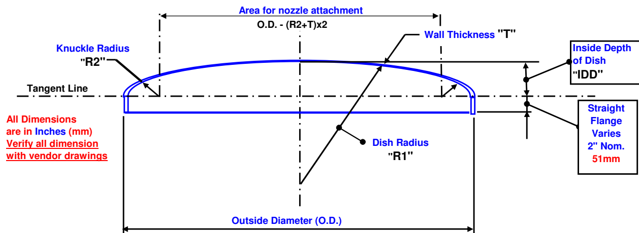
Millimeters (Flanged & Dished Head Table)
