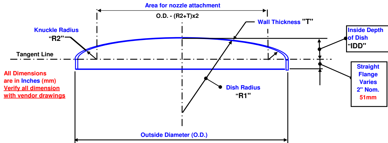
Inches (Flanged & Dished Head ASME Table)
