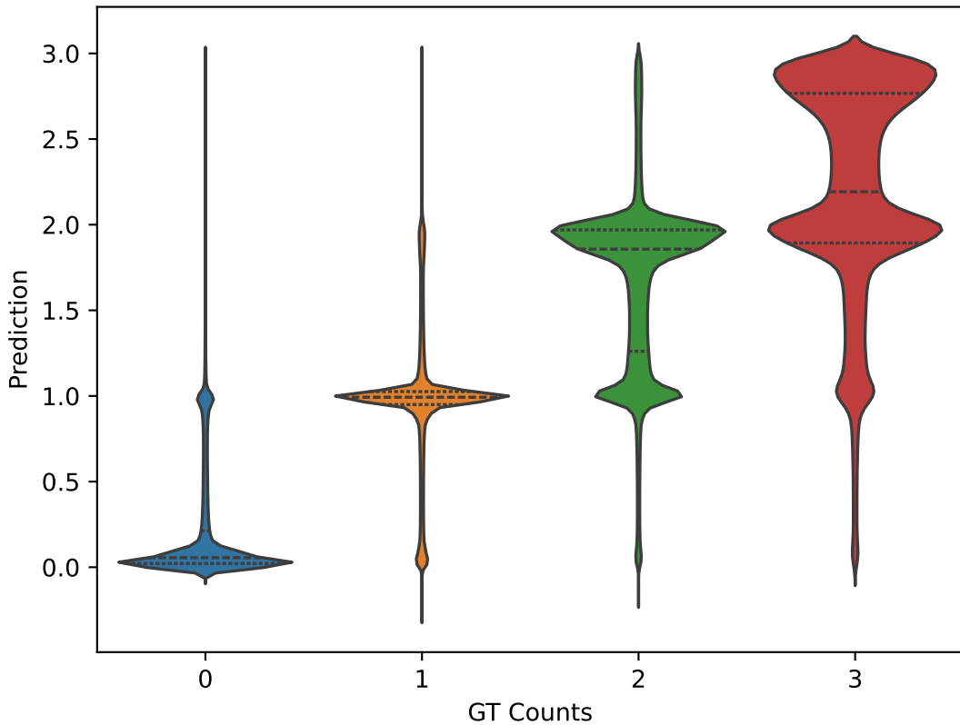
Clemson Dom GT vs Prediction
