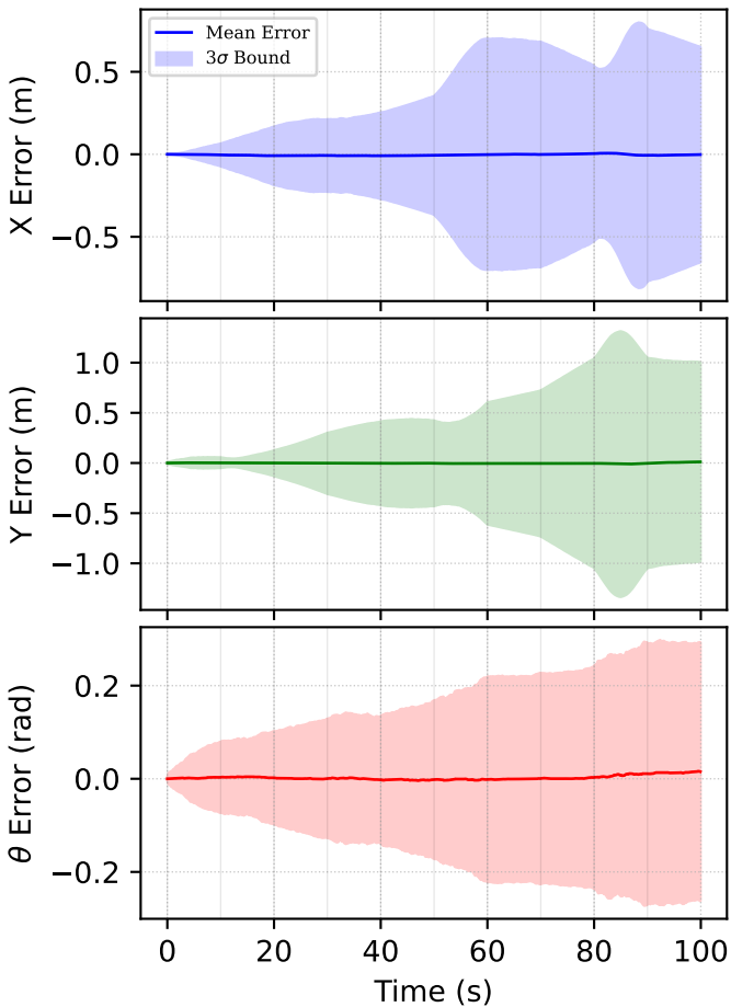
State Error Evolution (N=100)
