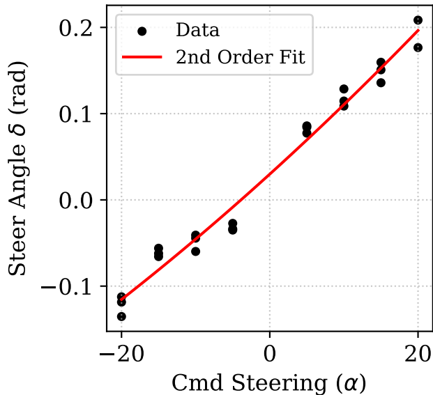
Steering Calibration
