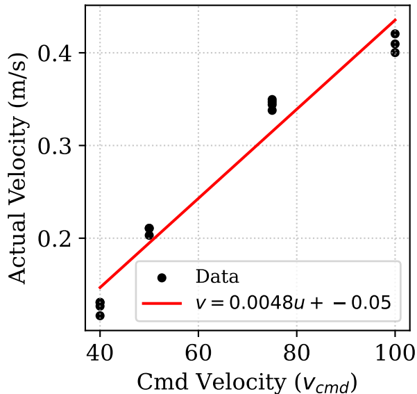
Velocity Calibration
