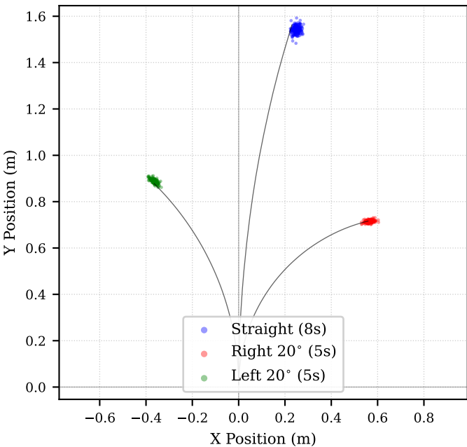
Motion Model Sampling (N=200)
