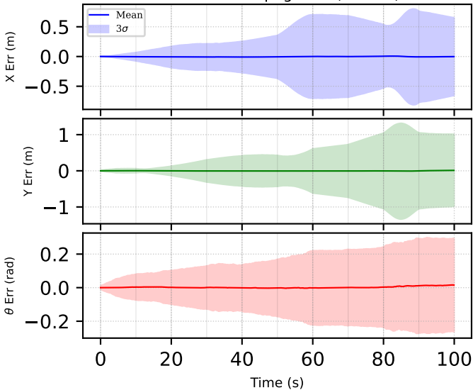
State Error Propagation (N=100)
