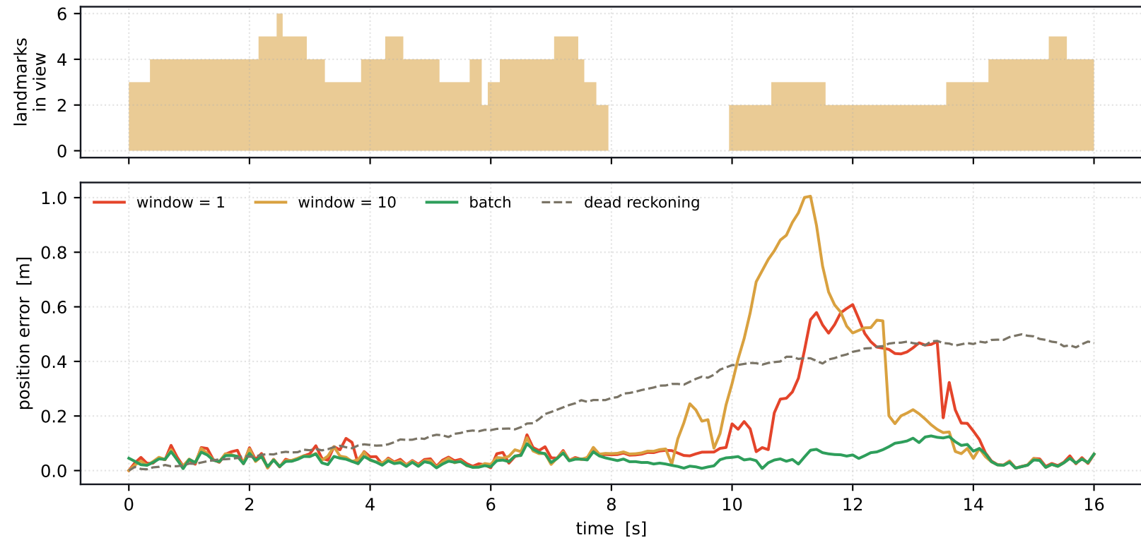
Uncertainty is driven by how many landmarks are in view
