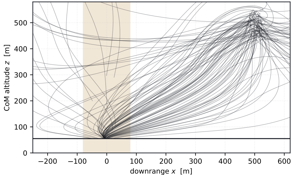
PD baseline, 120 recorded descents
