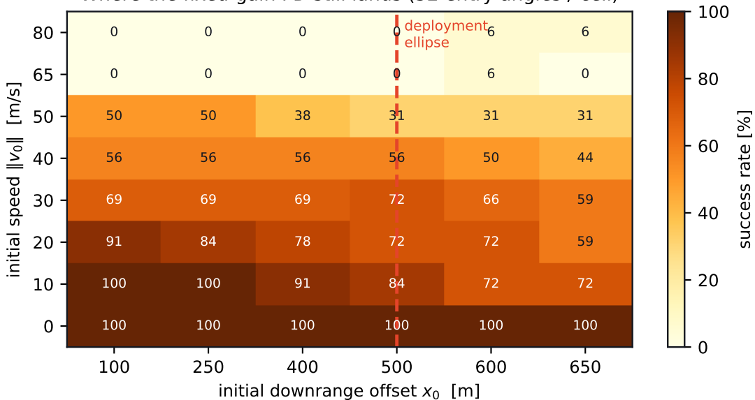
Where the fixed-gain PD still lands (32 entry angles / cell)
