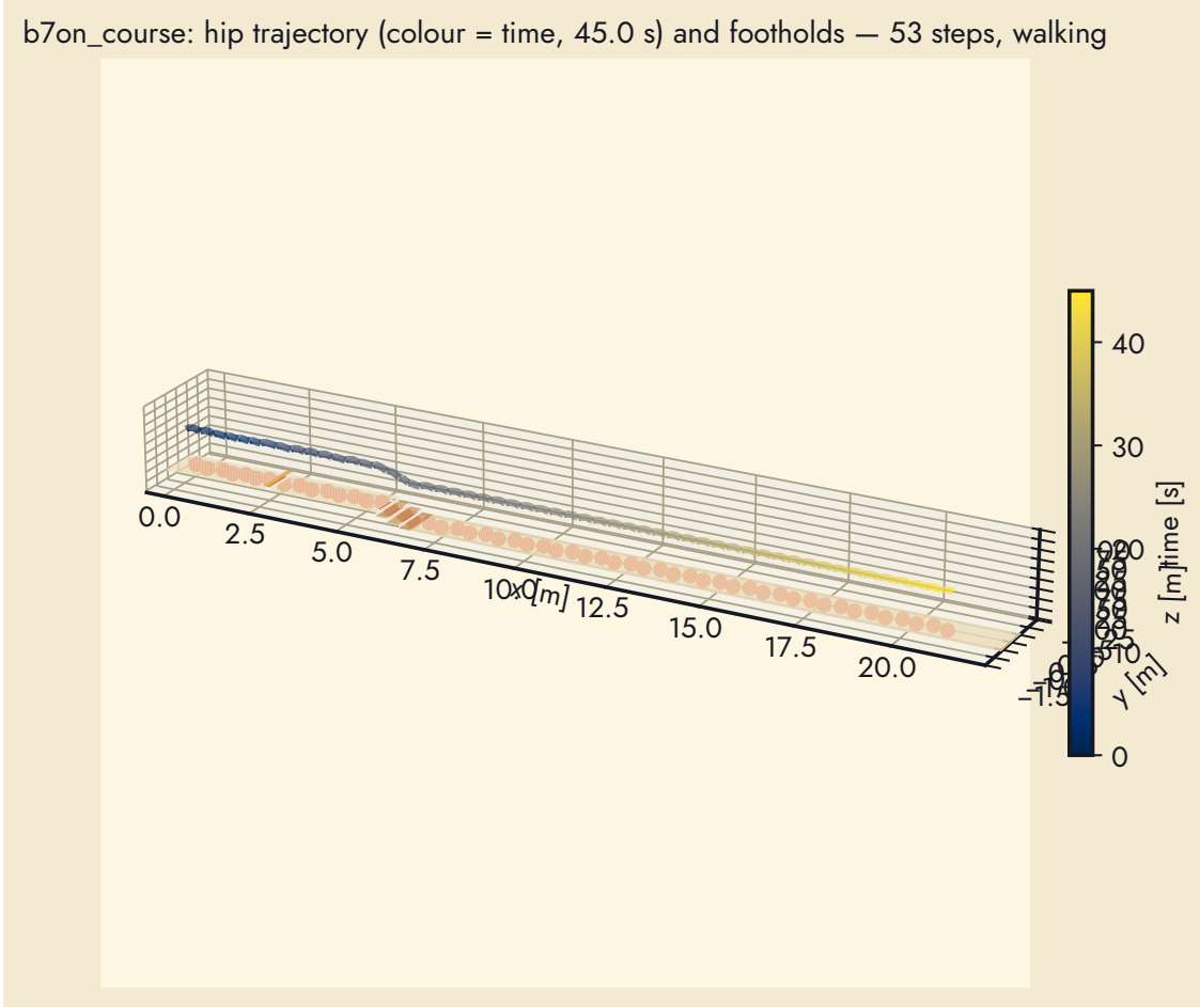
Figure 22: Footed biped with perception in the loop on the combined course: hip trajectory (colour = time) and footholds over the crate and down the staircase.
