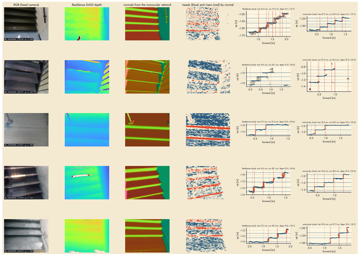
Figure 1: Per scene: RGB, RealSense depth, monocular normals, tread/riser labels from the normals, and the side profile of a 0.5m band of the cloud with the fitted tread (blue) and riser (red) lattices, for the RealSense and the monocular cloud.
