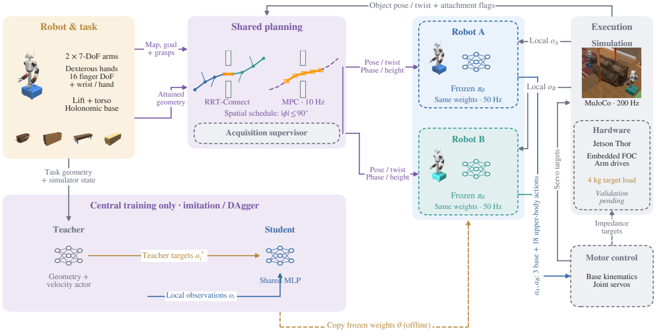
Fig. 2. Shared planning and local execution. Signal names are placed on arrows; blocks identify computations. Shared pose/twist, phase and height references reach both frozen actors, while o_i contains only that robot’s joint/hand feedback and object-relative observations. Central imitation/DAGger uses teacher action labels; dashed weight copying occurs offline. Motor conversion supplies servo targets in simulation and impedance targets to the hardware interface. Hardware system validation remains pending.
