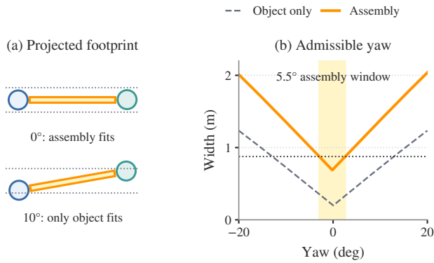
Fig. 7. Why the grasp changes passage feasibility. Analytic projections use the measured beam handoff geometry (seed 142024). (a) Dashed bounds show the available opening width after the 22 mm search margin on each side; the circles are base footprints. (b) The object-only yaw range is about 25.8^\circ , versus 5.5^\circ for the assembly (shaded); the horizontal dotted line is the door budget.
