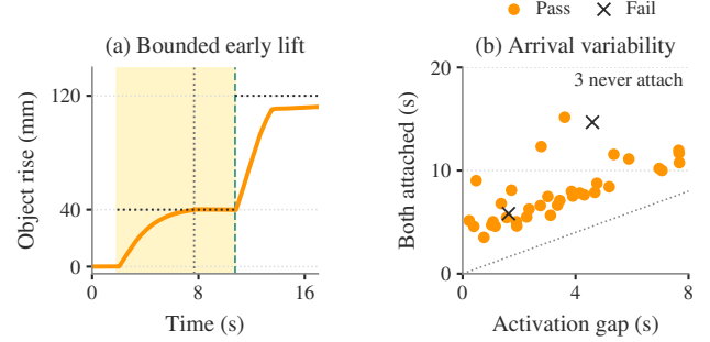
Fig. 2. Independent arrival. (a) Loading dock, seed 142013; measured object rise under a 7.68 s activation gap. Shading marks early lift; vertical dotted/dashed lines mark late activation/second attachment; horizontal lines mark height targets. (b) Both-attachment times for the 37 trials that acquire the object; color marks final mission outcome. The other three trials never attach both robots. The diagonal is t = \Delta .
