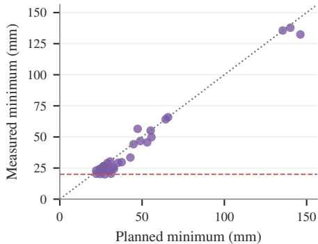
(b) 31 doorway passes
