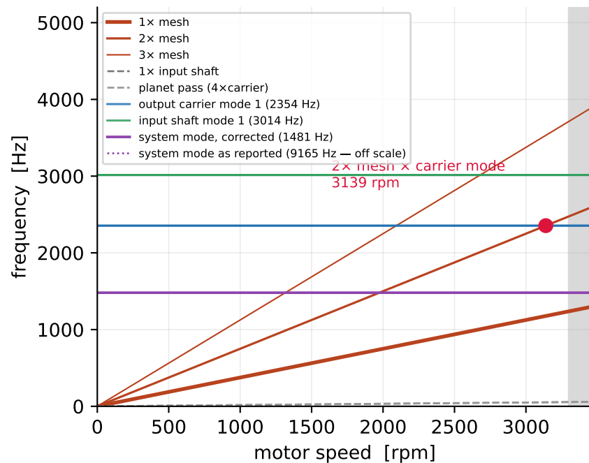
(b) Campbell diagram, 0 - redline
