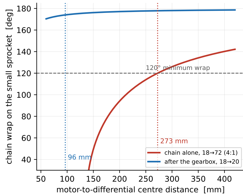
(a) why a gearbox at all
