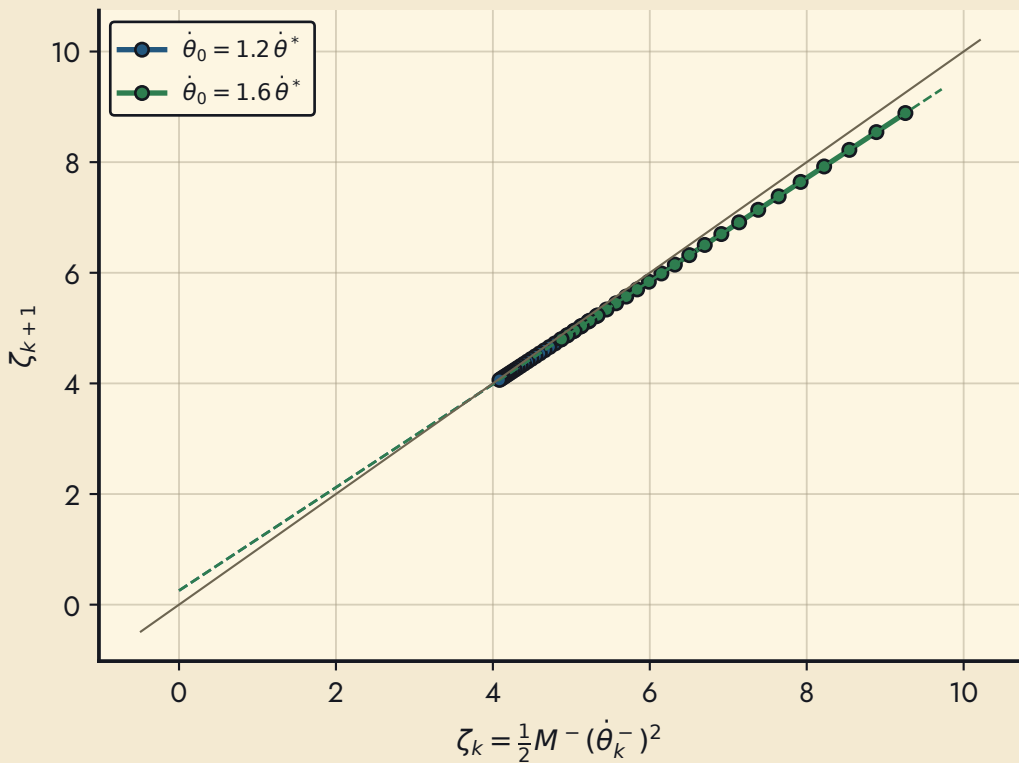
Return map of \dot{\theta}^- : simulation vs. the analytic slope \delta^2/M^-
