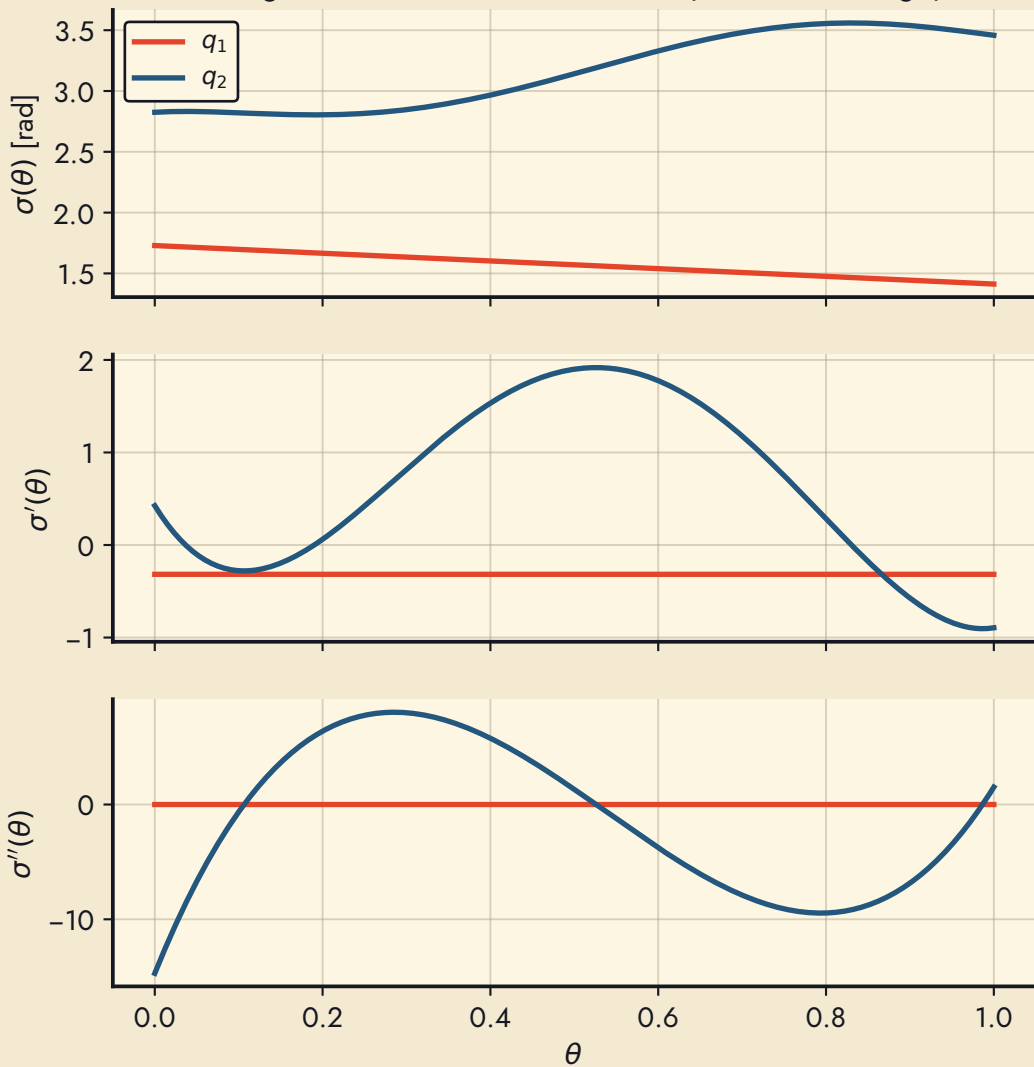
Flat ground: \sigma(\theta) and derivatives (ECE1658 design)
