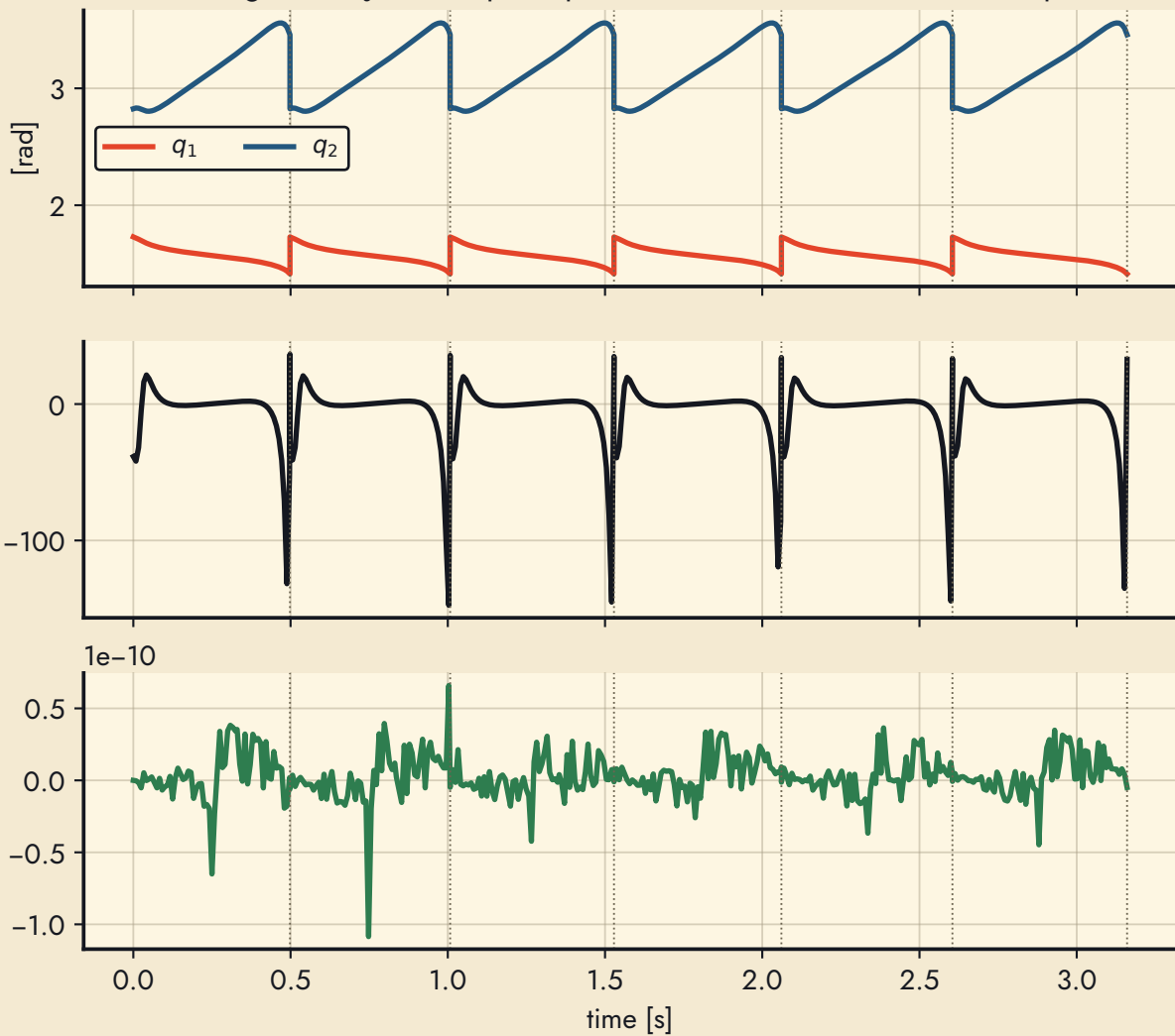
Flat ground: joints, hip torque and constraint error over 6 steps
