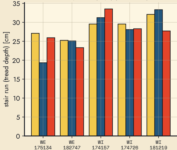
stair run (tread depth): pipeline vs tape
