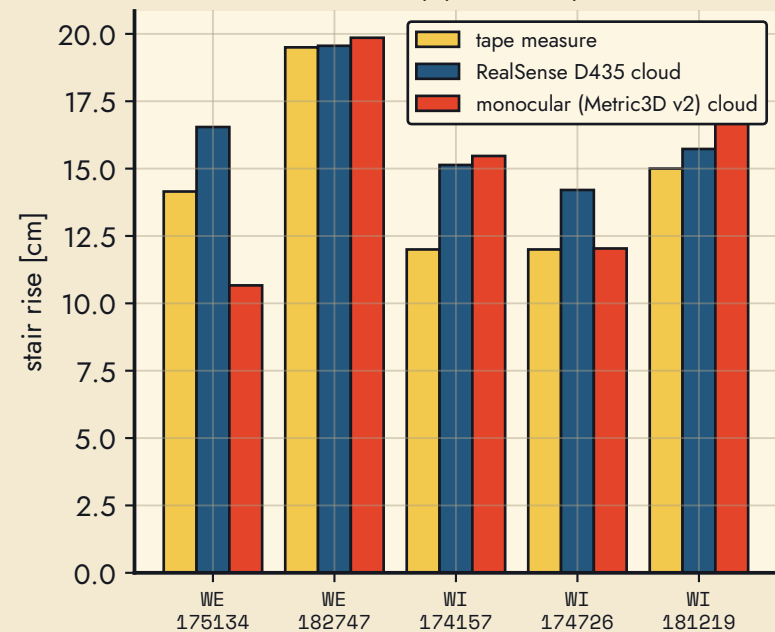
stair rise: pipeline vs tape
