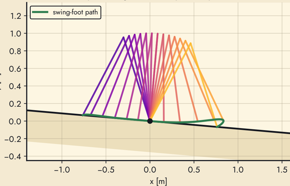
slope -5 deg, course impact map, k = 6
