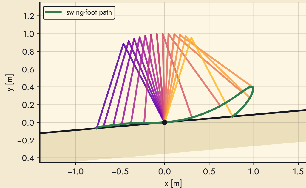
slope +5 deg, course impact map, k = 8
