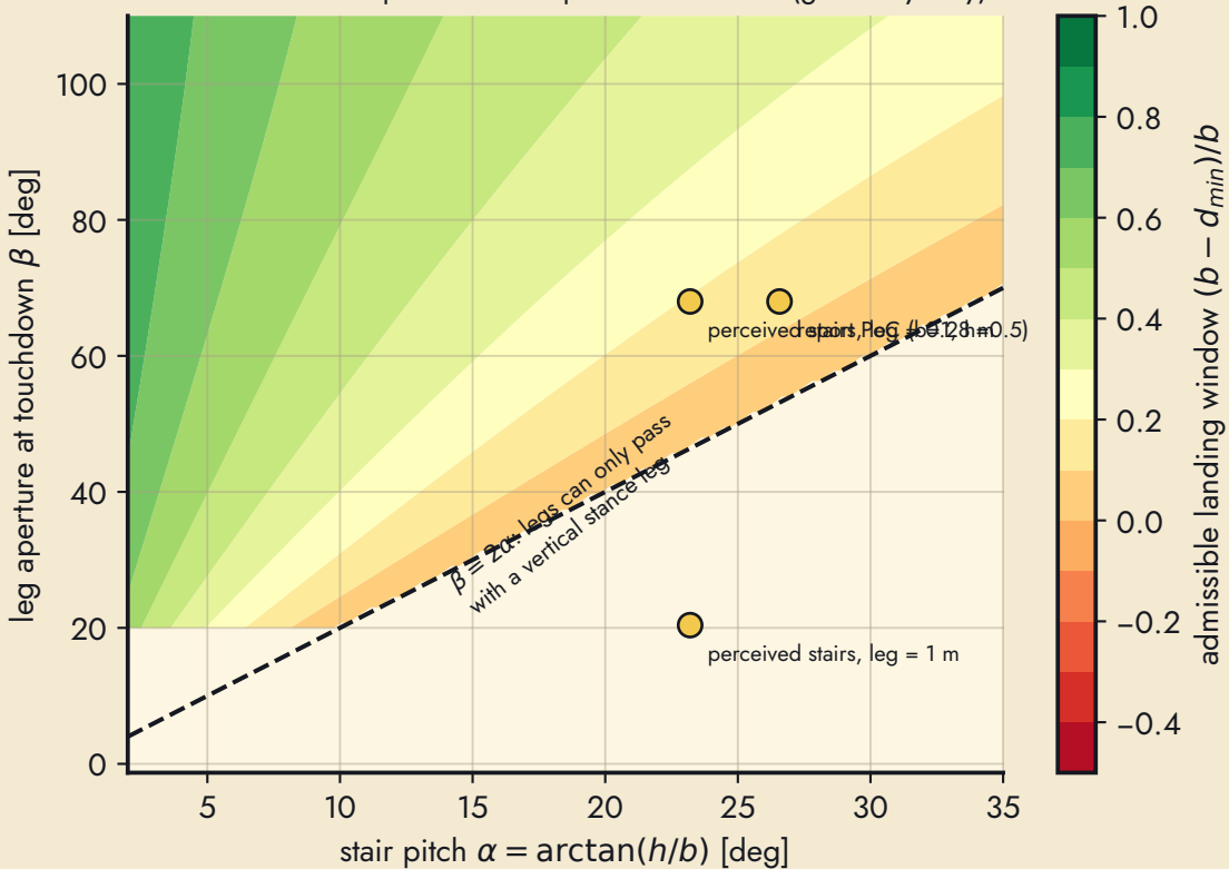
Which stairs can a point-foot compass walker take? (geometry only)
