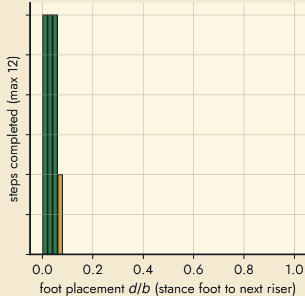
descending 5 deg stairs ( b = 0.76 m, h = 0.067 m), course impact map
