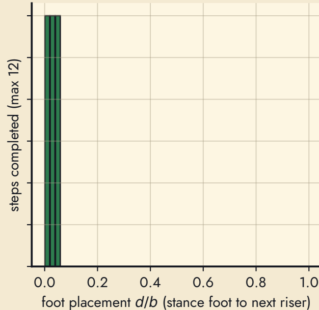
descending 10 deg stairs ( b = 0.75 m, h = 0.133 m), course impact map
