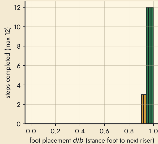
ascending 5 deg stairs ( b = 0.76 m, h = 0.067 m), course impact map
