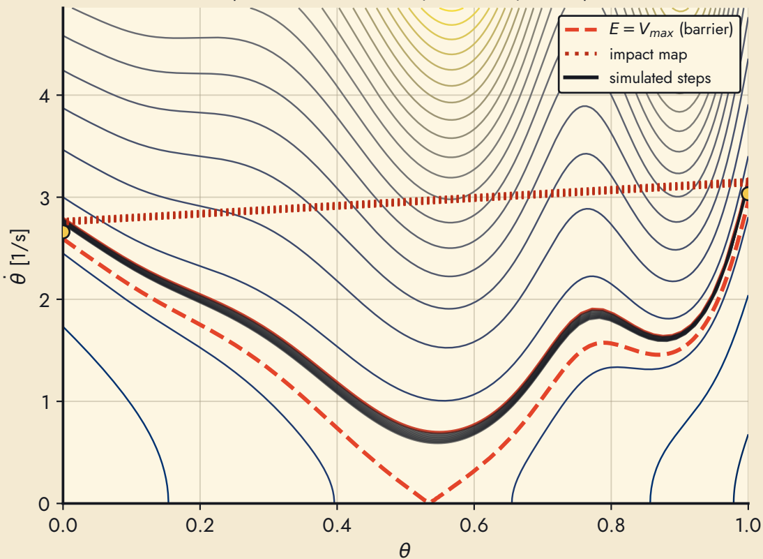
slope +5 reflect on stairs ( d = 0.97 b): 12 steps
