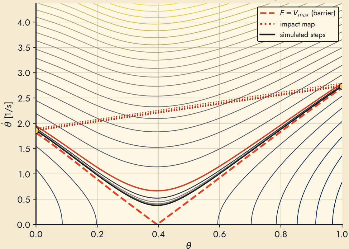
slope -10 kinematic on stairs ( d = 0.03 b): 12 steps
