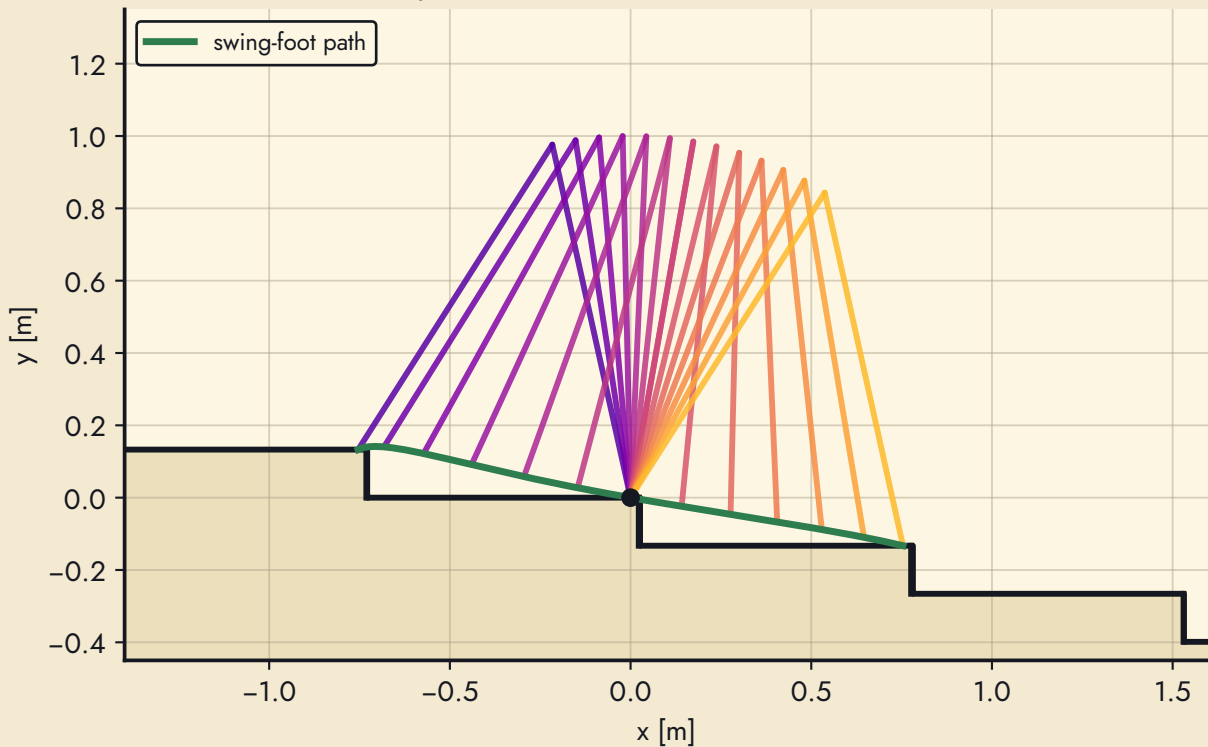
slope -10 kinematic on stairs, d = 0.03 b
