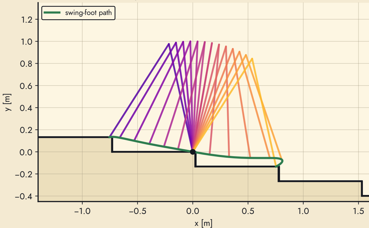
slope -10 reflect on stairs, d = 0.03 b
