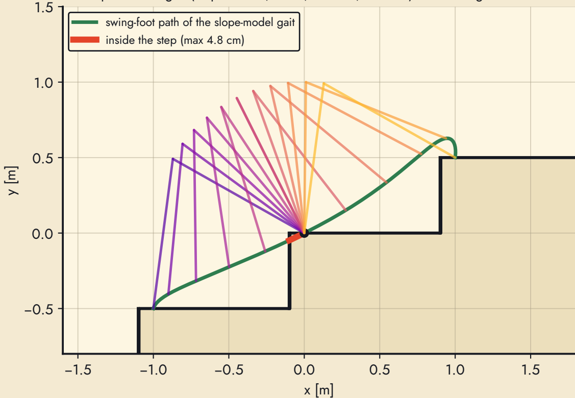
The report's stair gait (slope model, b = 1 , h = 0.5 , d = 0.9 ) checked against real treads
