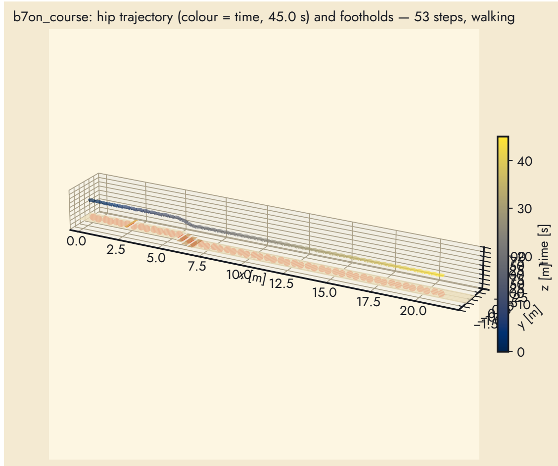
Figure 22: Footed biped with perception in the loop on the combined course: hip trajectory (colour = time) and footholds over the crate and down the staircase.
