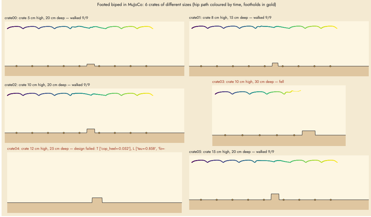
Figure 21: The crate runs: the leading step lands 5 cm past the crate and the trailing step returns to the regular gait’s landing state.
