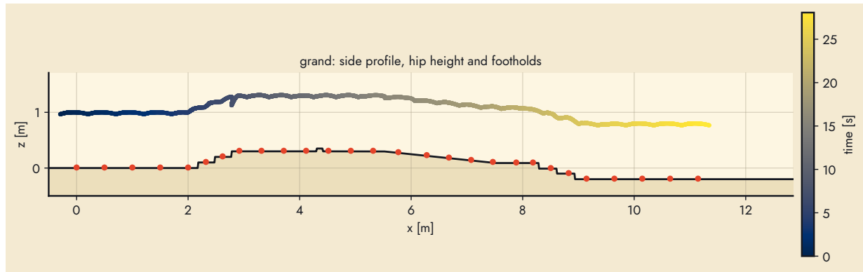
Figure 23: The long course in MuJoCo: terrain profile, hip height (colour = time) and the footholds, from the flat approach through the staircase, the crate, the ramp and the descent.
