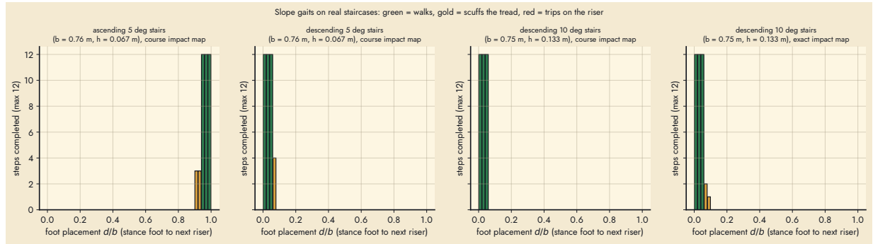
Figure 11: Slope gaits on real staircases: steps completed (of 12) versus foot placement d/b .
