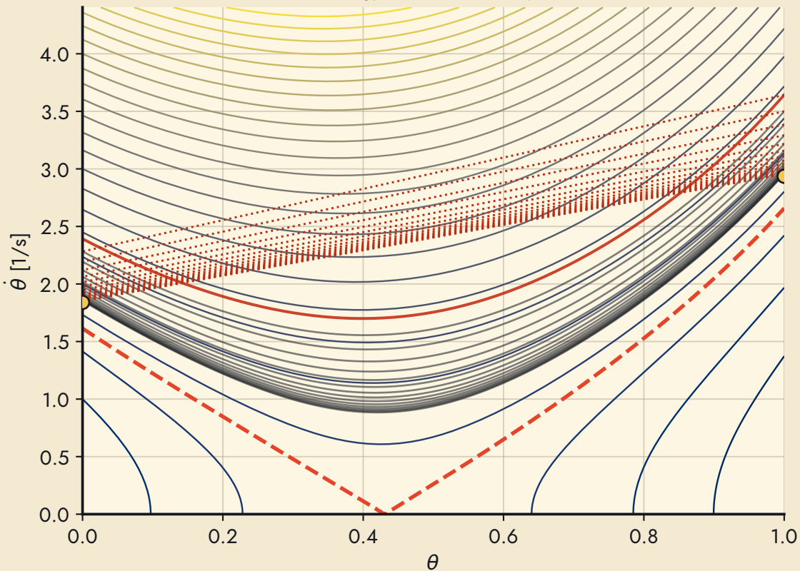
Five-link, flat: energy levels and 16 steps from 1.3 \dot{\theta}^*
