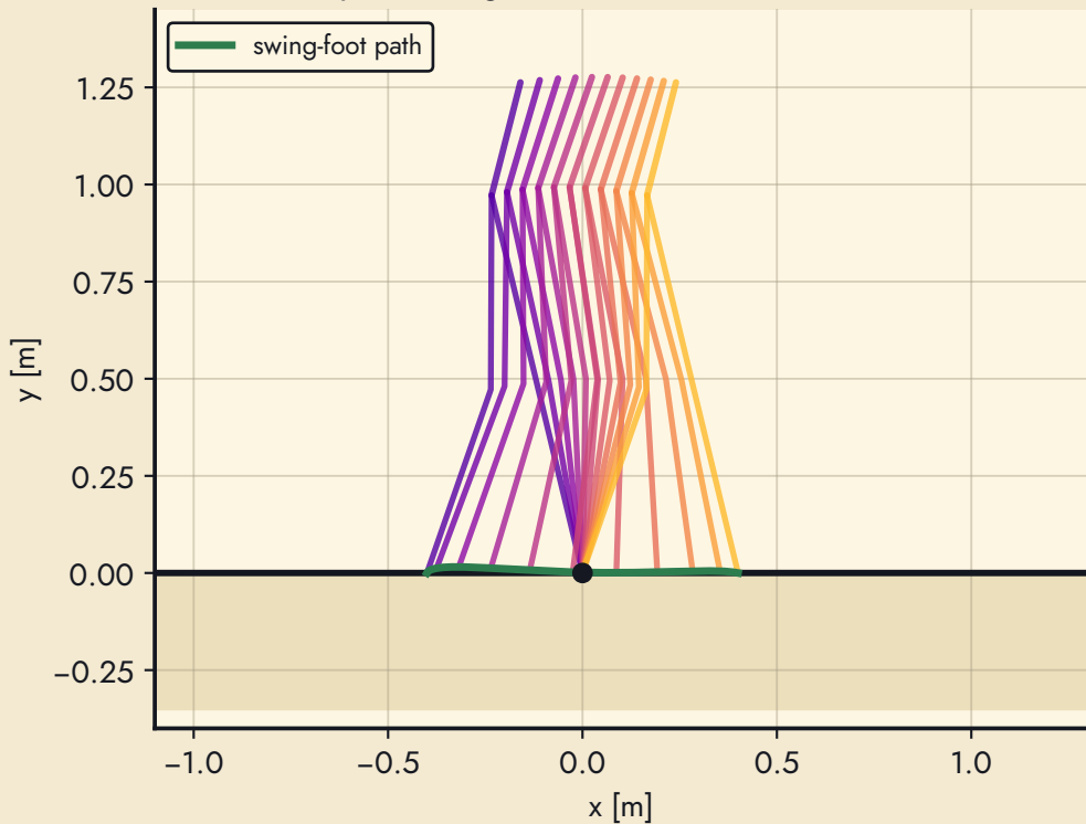
Five-link biped, flat ground: constraint set (stride 0.40 m)
