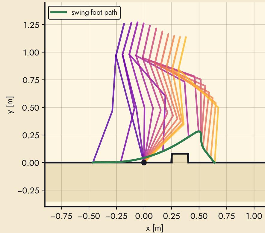
case 0: leading leg over the box (0.64 m step)
