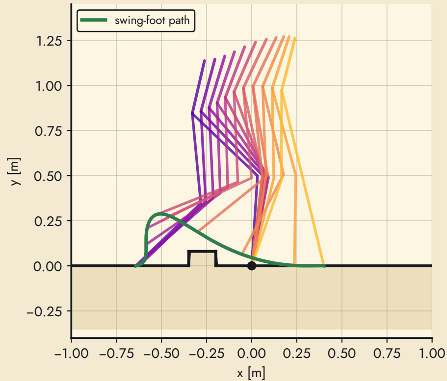
case 0: trailing leg over the box (0.40 m step), then the recovery step
