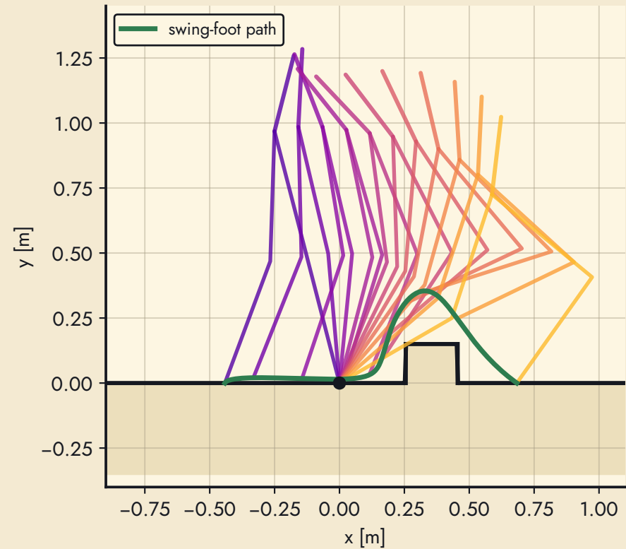
case 1: leading leg over the box (0.68 m step)
