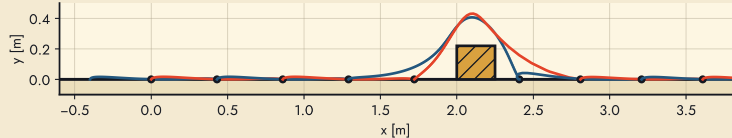
case 2: swing-foot paths of the whole plan (perceived box 1.99 m / 23 cm / 23 cm; true 2.00 / 25 / 22)
