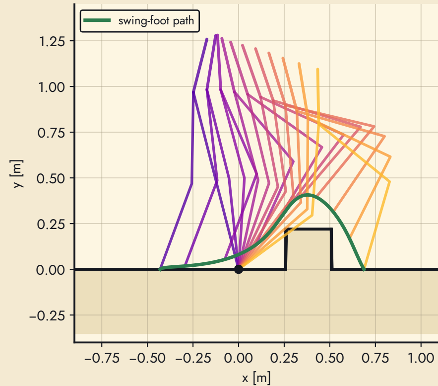
case 2: leading leg over the box (0.69 m step)
