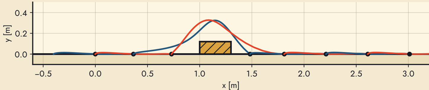
case 3: swing-foot paths of the whole plan (perceived box 1.00 m / 28 cm / 13 cm; true 1.00 / 30 / 12)
