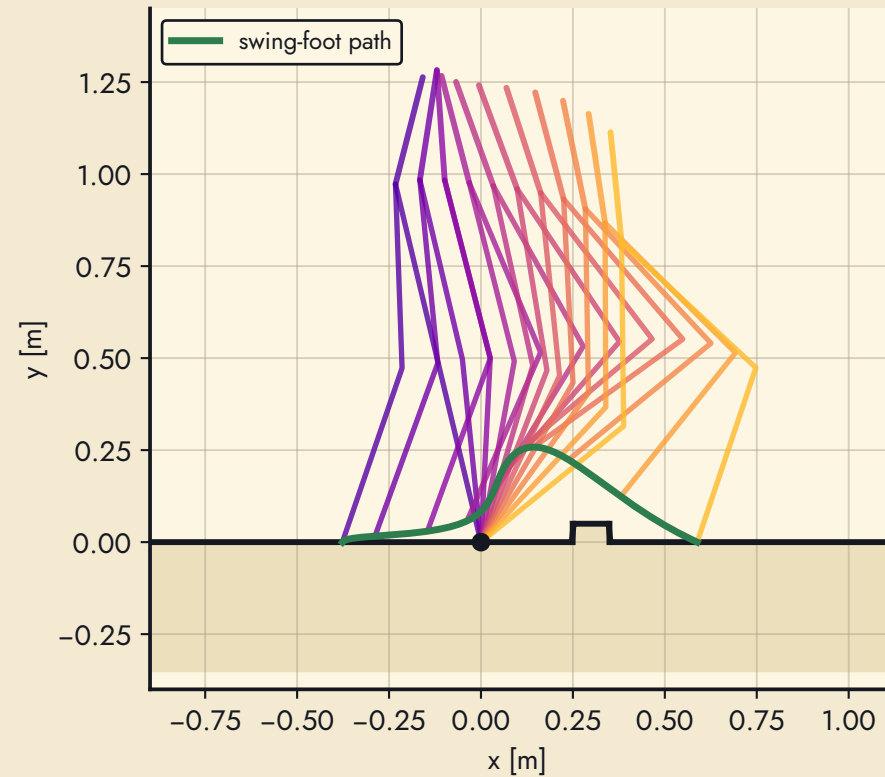
case 4: leading leg over the box (0.59 m step)
