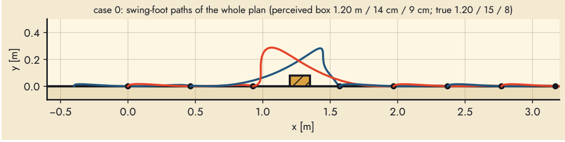
Figure 16: Case 0: swing-foot paths of the whole plan in world coordinates (alternating colours per step, dots = stance feet).
