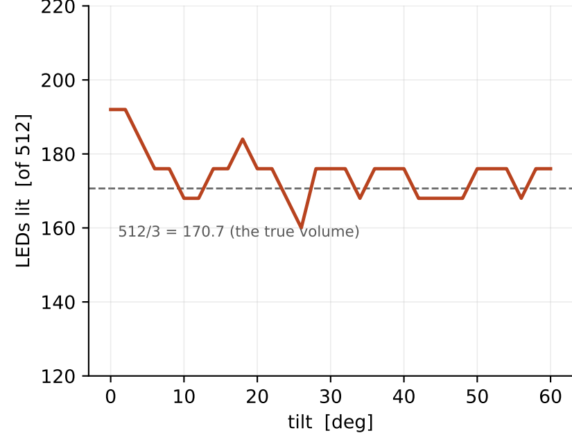
(c) quantisation: the display over-reads when flat
