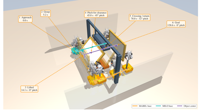
Fig. 1. Verified pitching-orientation rollout. MABEL and MILO carry the 1.5 kg panel through a constrained passage with the geometric SE(3) RRT-Connect/Jacobian-rate teacher. Colored trajectories show the two measured base motions and object center. Saved robot and payload poses are overlaid under one fixed camera; numbered timestamps label the approach, grasp, lift, pitch, obstacle crossing and final state. The complete run lasts 128.6 s, reaches 45.2° measured pitch and keeps maximum base tilt at 0.16°.
