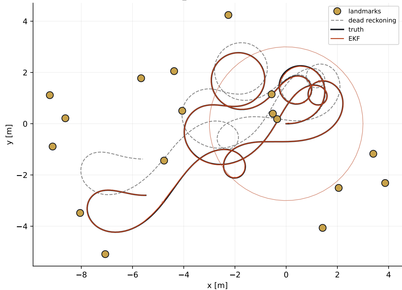
Lost in the Woods, r_{\text{max}} = 3 \text{ m} — 3\sigma ellipses every 4.5 s
