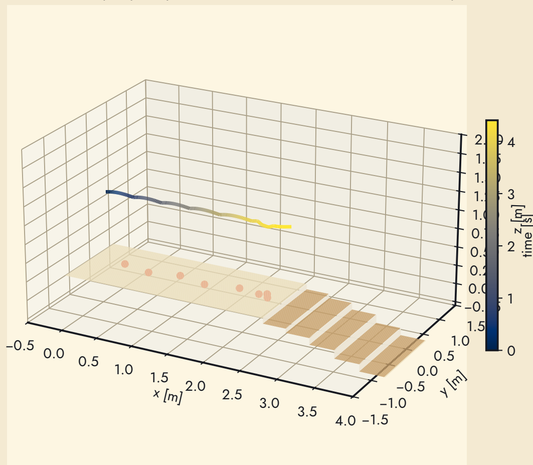
Stairs down #10: hip trajectory (colour = time, 4.4 s) and footholds — 7 steps, fell
