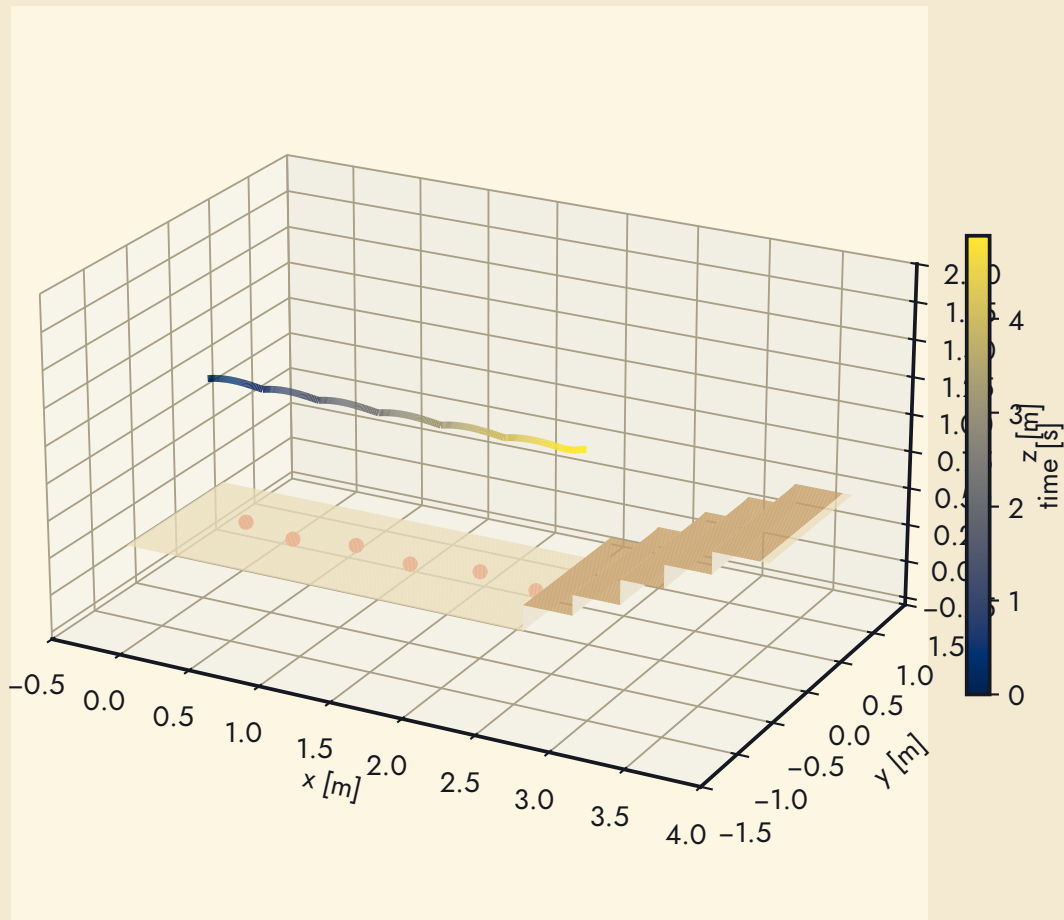
Stairs up #4: hip trajectory (colour = time, 4.9 s) and footholds — 5 steps, fell
