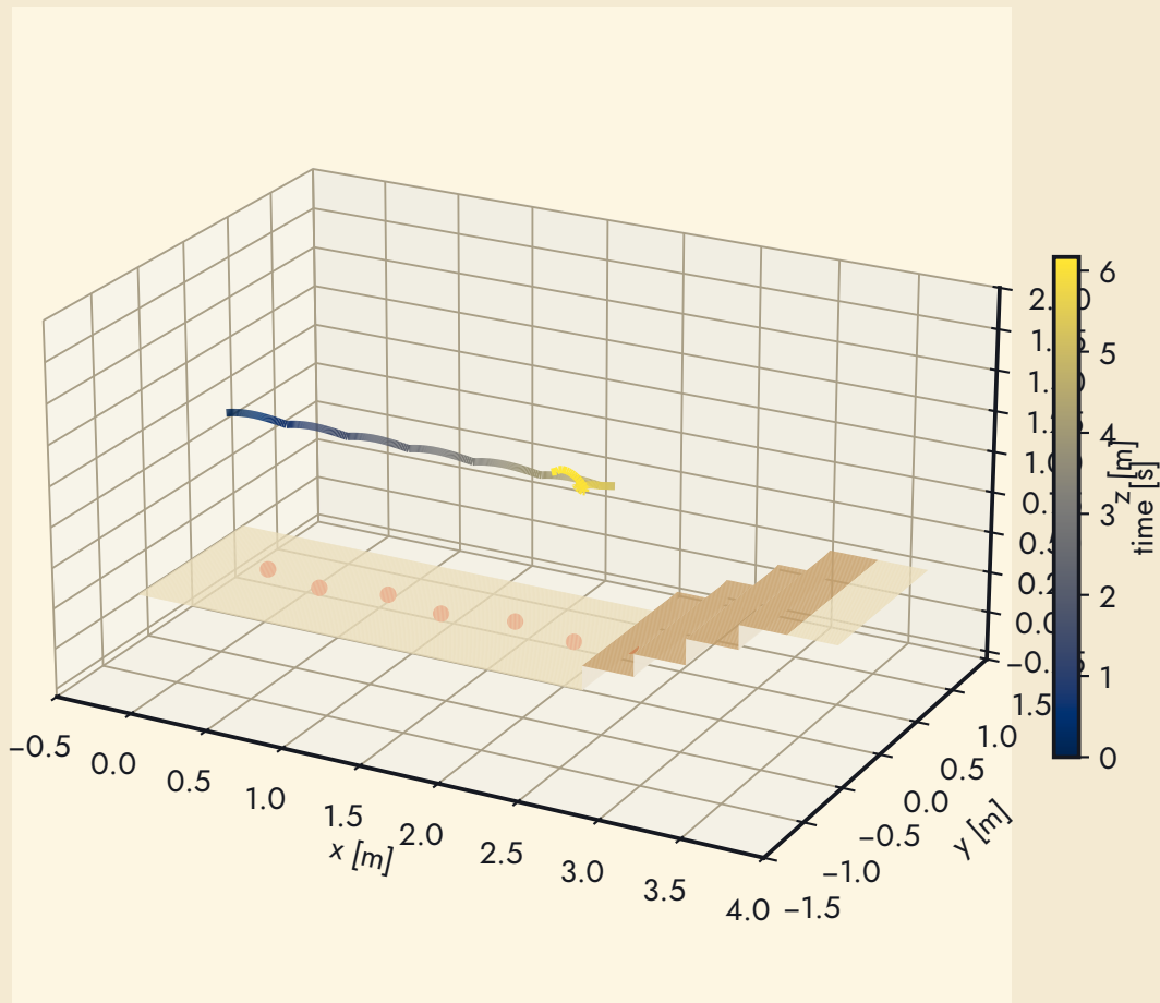
Stairs up #9: hip trajectory (colour = time, 6.2 s) and footholds — 6 steps, fell
