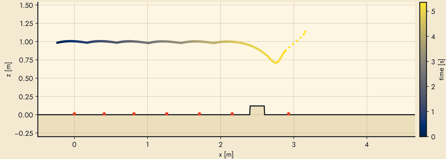
box: side profile, hip height and footholds
